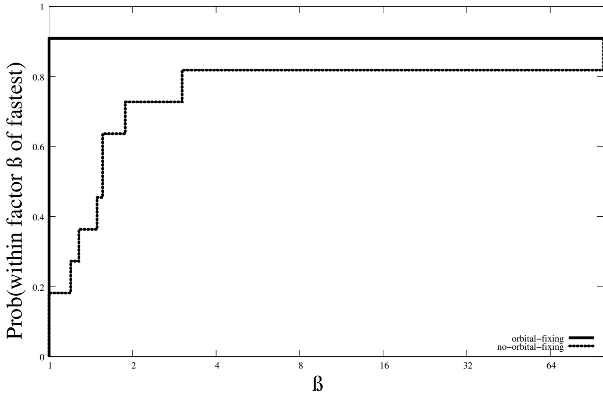
Figure 2: Performance Profile of Impact of Orbital Fixing
