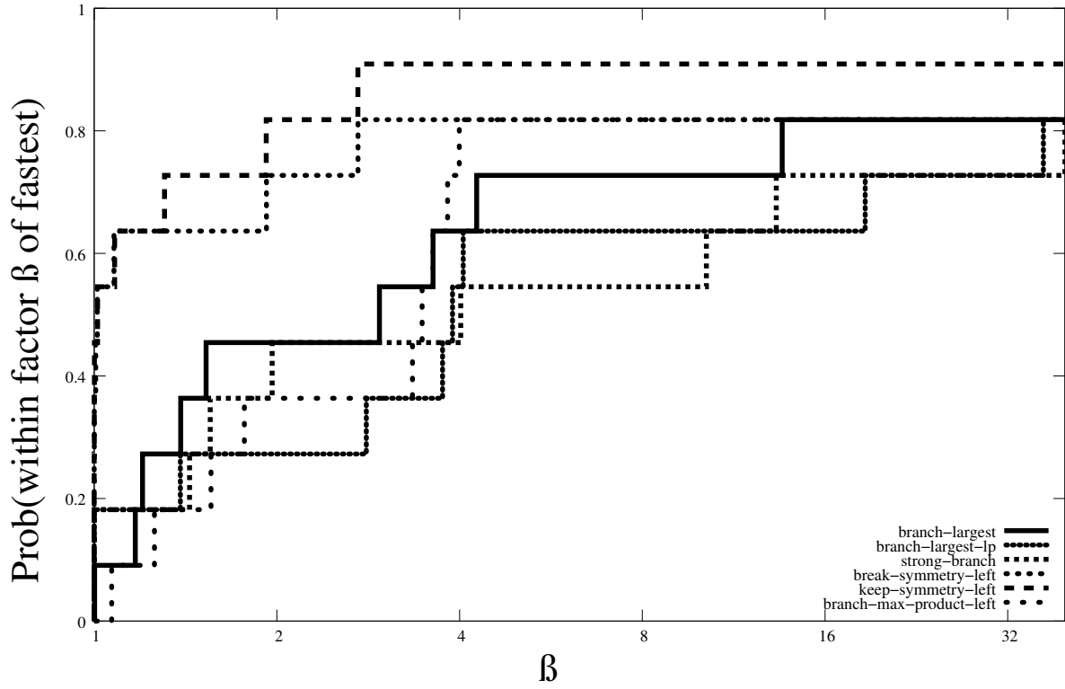
Figure 1: Performance Profile of Branching Rules
