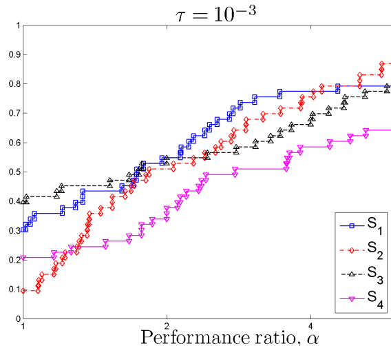
Figure 2.1: Sample performance profile \rho_s(\alpha) (logarithmic scale) for derivative-free solvers.
