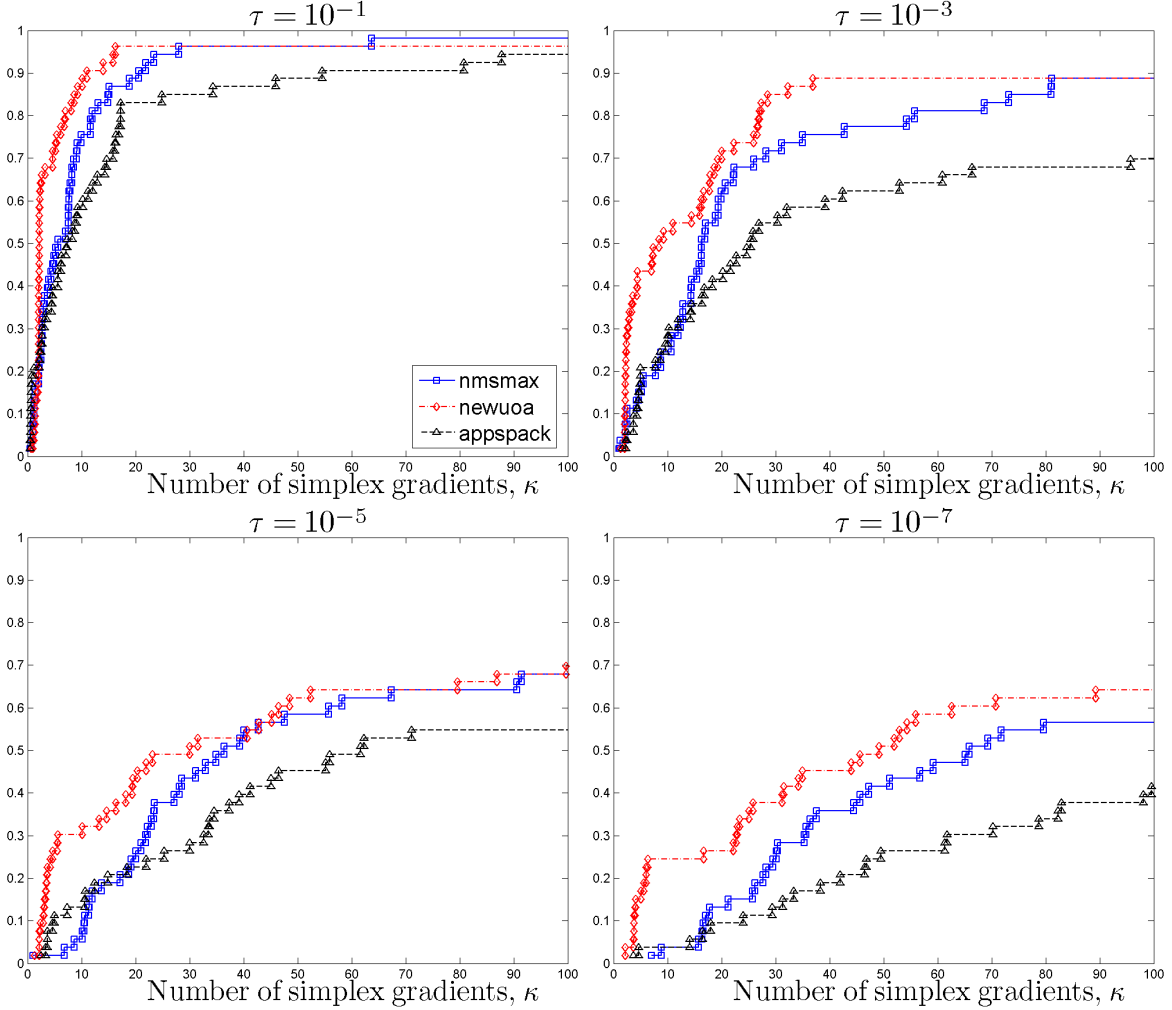
Figure 5.3: Data profiles d_s(\kappa) for the noisy problems \mathcal{P}_N show the percentage of problems solved as a function of a computational budget of simplex gradients.
