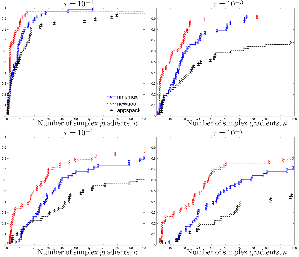
Figure 5.1: Data profiles d_s(\kappa) for the smooth problems \mathcal{P}_S show the percentage of problems solved as a function of a computational budget of simplex gradients.
