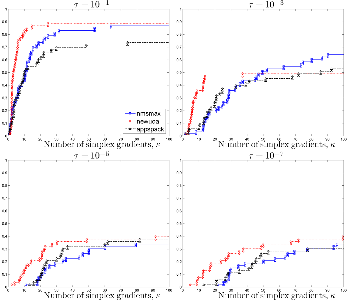
Figure 5.5: Data profiles d_s(\kappa) for the piecewise-smooth problems \mathcal{P}_{PS} show the percentage of problems solved as a function of a computational budget of simplex gradients.
