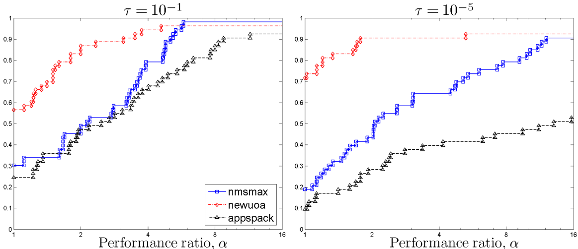
Figure 5.2: Performance profiles \rho_s(\alpha) (logarithmic scale) for the smooth problems \mathcal{P}_S .
