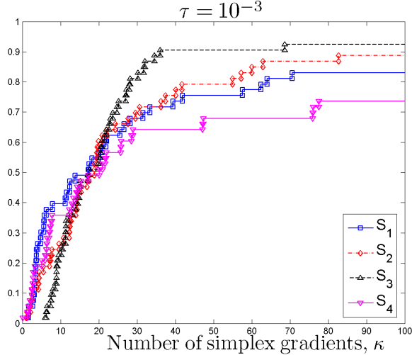
Figure 2.2: Sample data profile d_s(\kappa) for derivative-free solvers.
