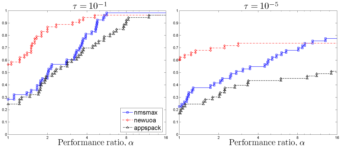
Figure 5.4: Performance profiles \rho_s(\alpha) (logarithmic scale) for the noisy problems \mathcal{P}_N .
