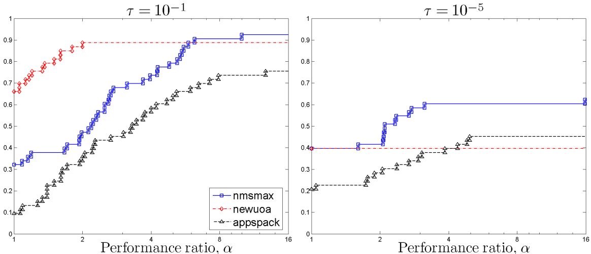
Figure 5.6: Performance profiles \rho_s(\alpha) (logarithmic scale) for the piecewise-smooth problems \mathcal{P}_{PS} .
