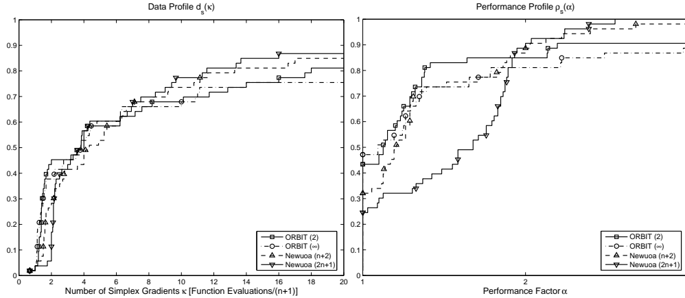
FIG. 5.3. Set \mathcal{P}_N of Noisy Test Problems: (a) Data Profile d_s(\kappa) Shows the Percentage of Problems Solved, \tau = .01 ; (b) Performance Profile \rho_s(\alpha) Shows the Relative Performance, \tau = .1 .
