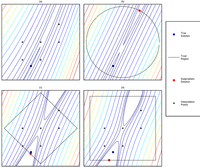
FIG. 2.1. Trust-Region Subproblem Solutions (all have same axes): (a) True Function, (b) Quadratic Taylor Model in 2-norm Trust-Region, (c) Quadratic Interpolation Model in 1-norm Trust-Region, (d) Gaussian RBF Interpolation Model in \infty -norm Trust-Region.
