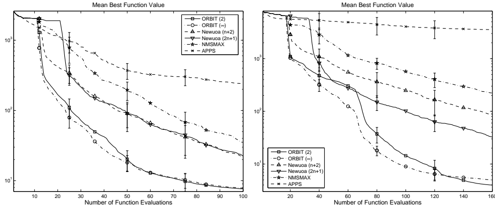
FIG. 5.1. Average of 30 Starting Points on Two Functions from \mathcal{P} ( \log_{10} scale, lowest line is best): (a) Extended Rosenbrock ( n = 10 ); (b) Extended Powell Singular ( n = 16 ).
