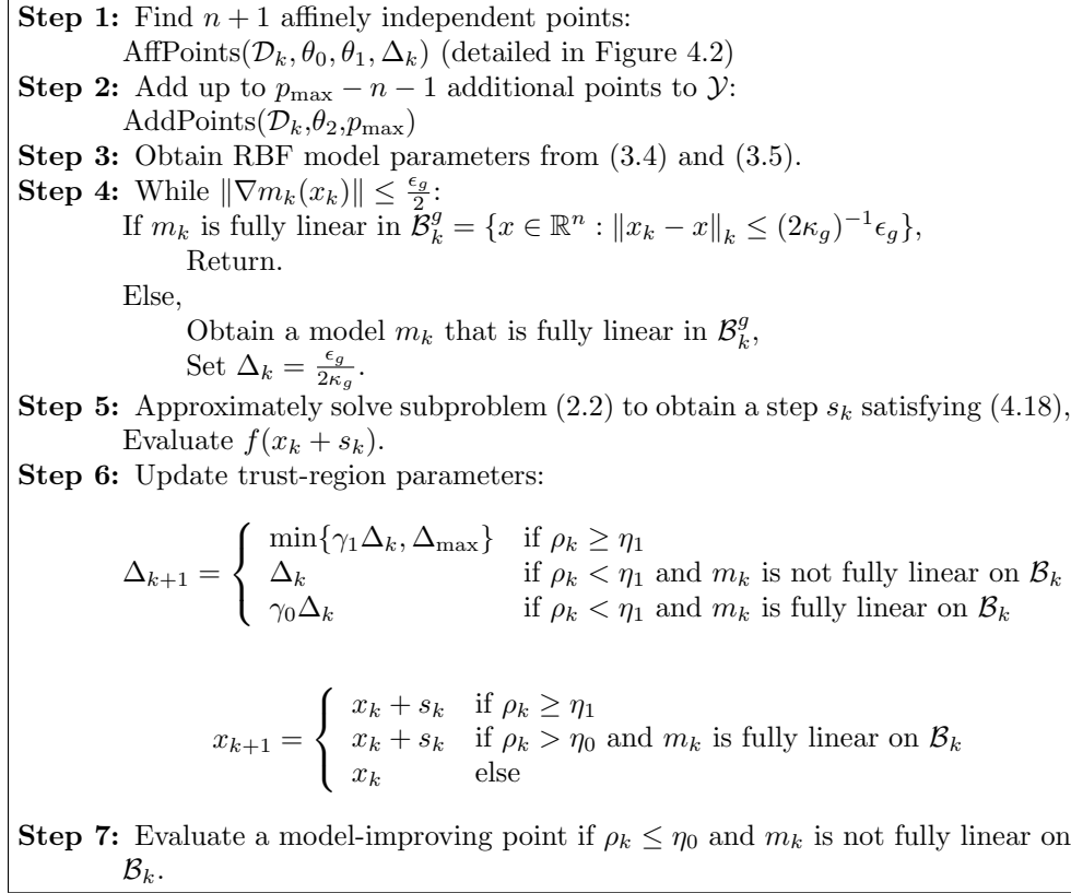
FIG. 4.1. Iteration k of the ORBIT Algorithm.
