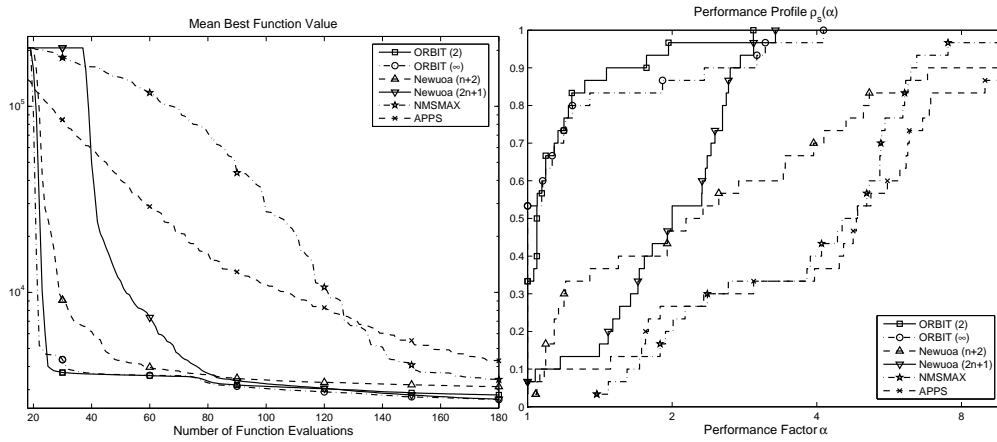
FIG. 6.2. GWB18 Problem ( n = 18 ): (a) ( \log_{10} scale) Mean Best Function Value (30 trials); (b) Performance Profile \rho_s(\alpha) Shows the Relative Performance, \tau = .01 .
