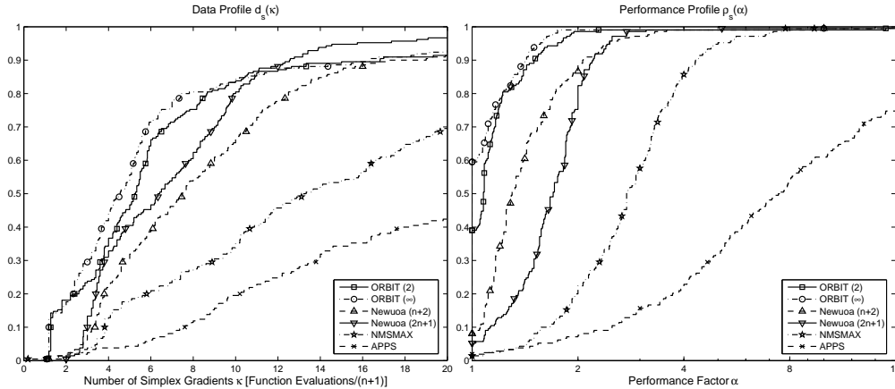
FIG. 5.2. Set \mathcal{P} of Smooth Test Problems: (a) Data Profile d_s(\kappa) Shows the Percentage of Problems Solved, \tau = .01 ; (b) Performance Profile \rho_s(\alpha) Shows the Relative Performance, \tau = .1 .
