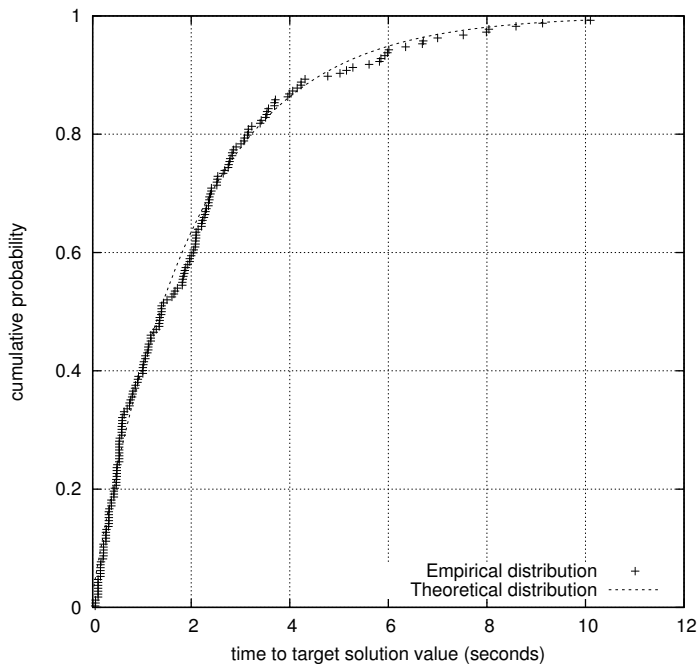
FIGURE 9. Superimposed empirical and theoretical distributions (times to target solution values measured in seconds on an SGI Challenge computer with 28 processors).
