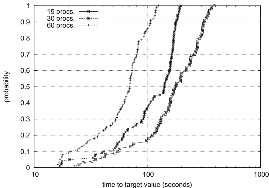
FIGURE 11. Time-to-target plots for the hierarchical distributed implementation of the GRASP with ILS heuristic for the diameter constrained minimum spanning tree on an instance with 100 nodes running on a grid environment using 15, 30, and 60 processors.
