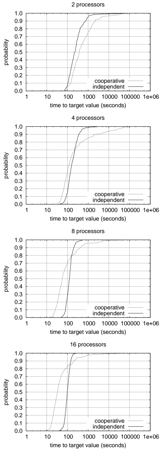
FIGURE 10. Empirical distributions of the time-to-target random variable for the independent and the cooperative parallelizations on 2, 4, 8, and 16 processors (target value set at 683).
