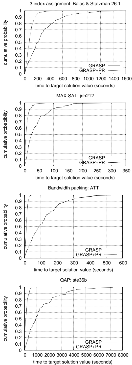
FIGURE 6. Time to target plots comparing running times of pure GRASP and GRASP with path-relinking on four instances of distinct problem types: three index assignment, maximum satisfiability, bandwidth packing, and quadratic assignment.
