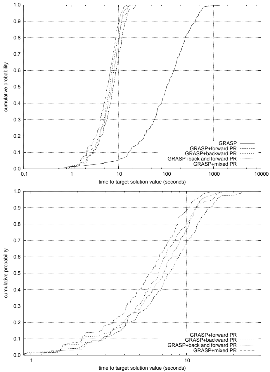
FIGURE 7. Time-to-target plots for pure GRASP and four variants of GRASP with path-relinking (forward, backward, back and forward, and mixed) on an instance of the 2-path network design problem.
