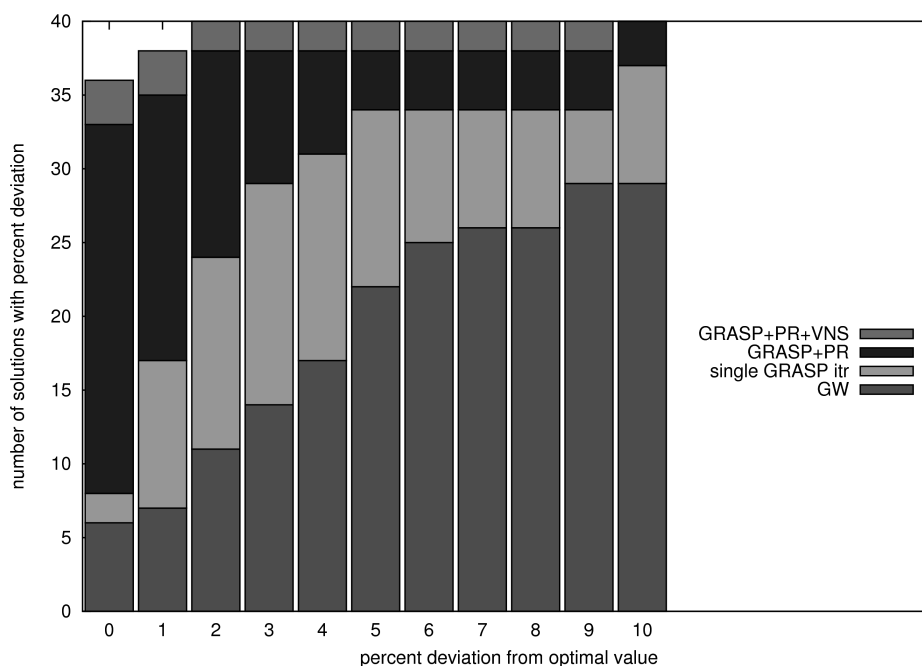
FIGURE 12. Performance of GW approximation algorithm, a single GRASP iteration (GW followed by local search), 500 iterations of GRASP with path-relinking, and 500 iterations of GRASP with path-relinking followed by VNS for series C prize-collecting Steiner tree problems.
