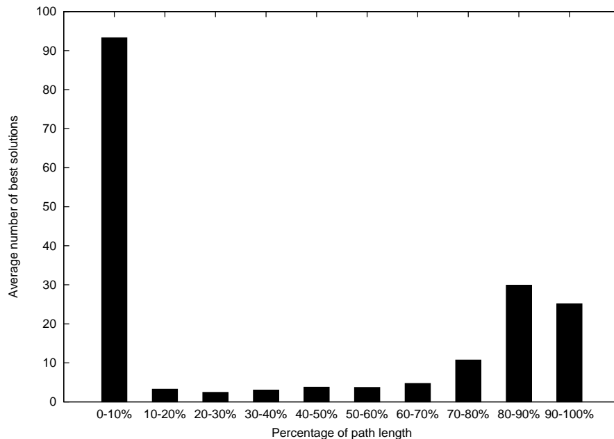
FIGURE 8. Average number of best solutions found at different depths of the path from the initial solution to the guiding solution on instances of the max-min diversity problem.
