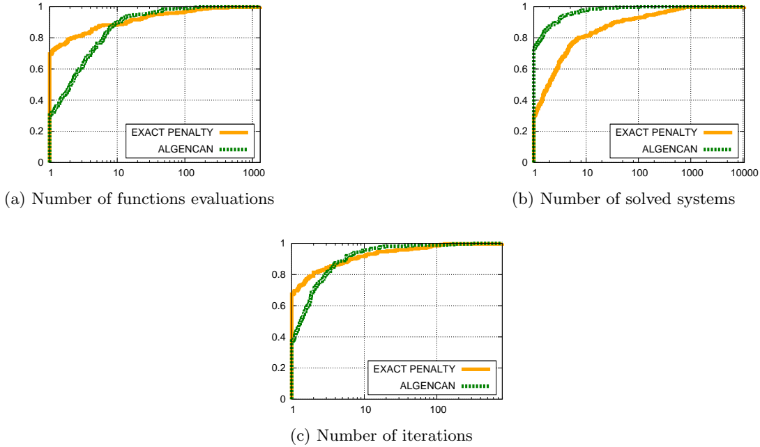
Figure 1: Performance profiles for the exact penalty algorithm and the ALGENCAN
