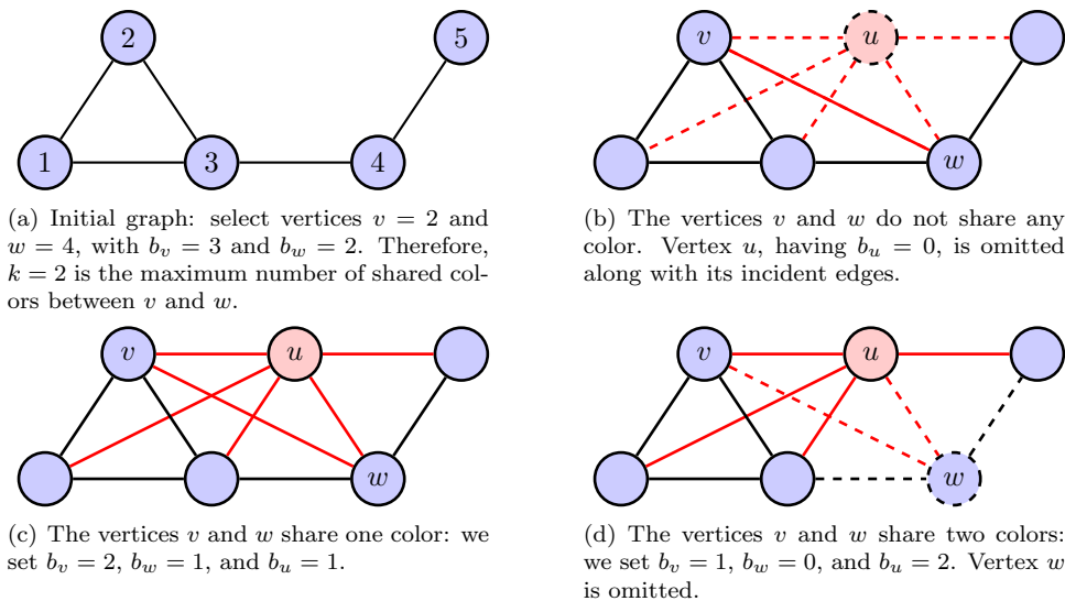
Figure 2: Example of the branching rule for the MIN-GMP problem: (a) the initial graph, and (b)–(d) the three branching nodes, when the vertices 2 and 4 are selected for branching.
