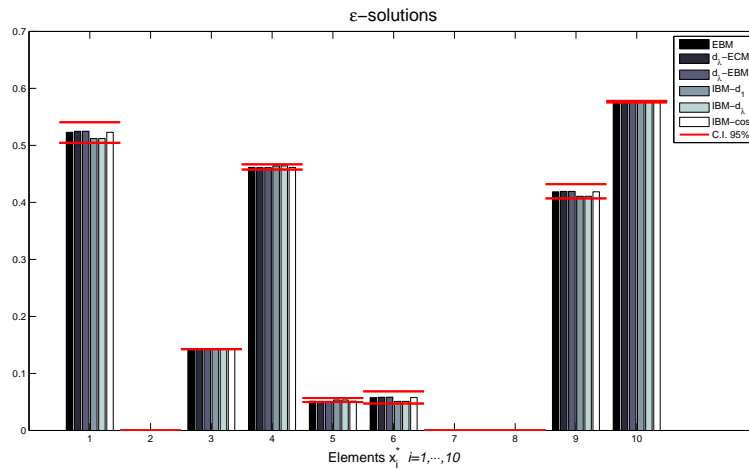
FIGURE 1. Confidence interval for SH10 first-stage solution.
