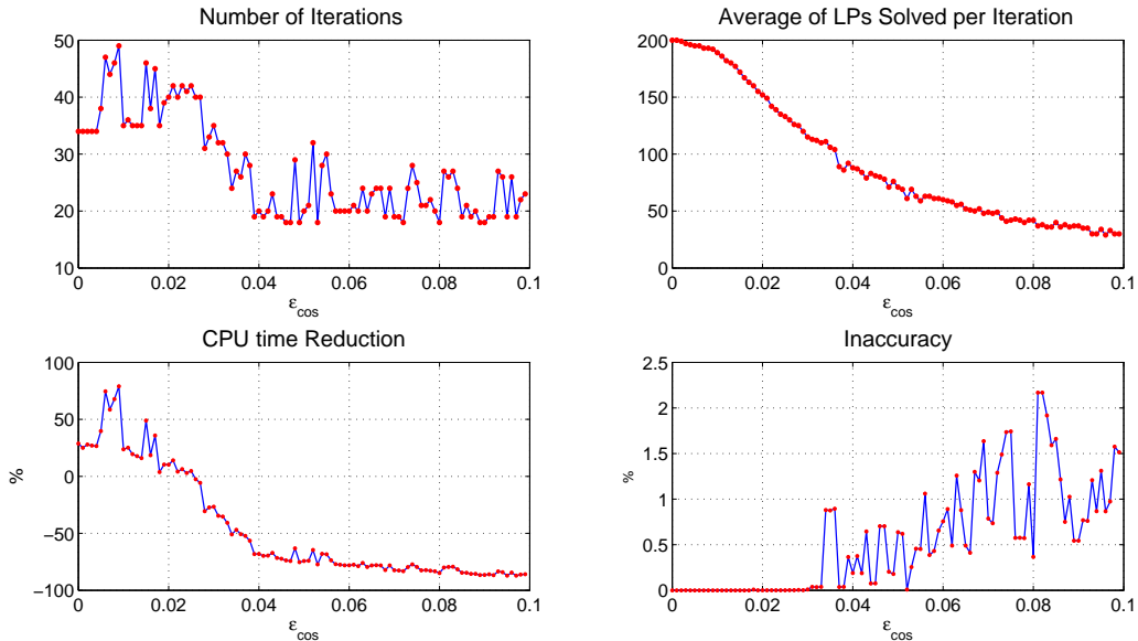
FIGURE 5. Sensitivity analysis for the Inexact Oracle 1.
