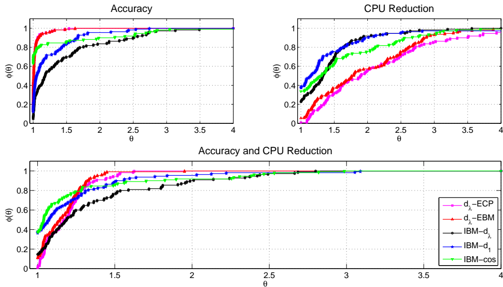
FIGURE 2. Performance profiles for all problems in the battery and all instances (110 runs).
