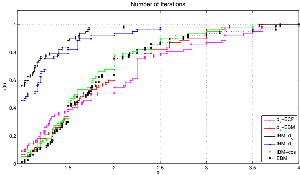
FIGURE 4. Performance profiles for problems with fixed recourse and fixed second-stage cost and all instances (77 runs).
