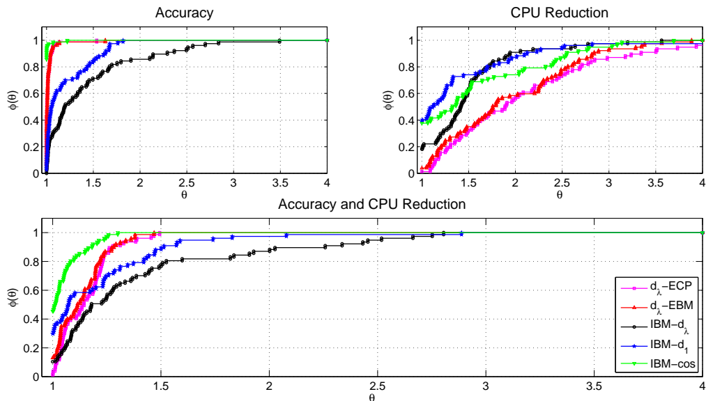
FIGURE 3. Performance profiles for problems with fixed recourse and fixed second-stage cost and all instances (77 runs).
