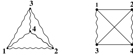
Figure 6: A homeomorph of K_4 and its two sides (cf. Lemma 5.8)
