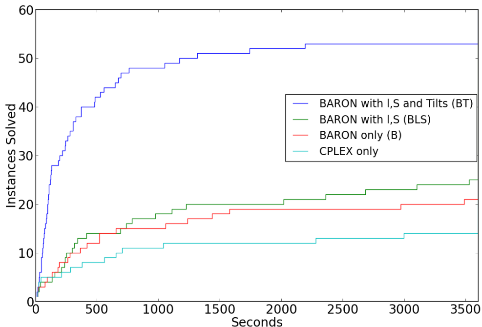
Figure 3: Cumulative distribution plots of solution times for the lot-sizing problem. The plots from top to bottom correspond to the order of the labels in the legend.
