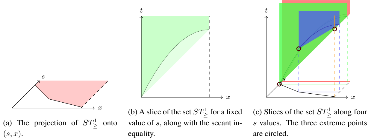
Figure 1: Visualizing the set ST_{\ge}^1 .
