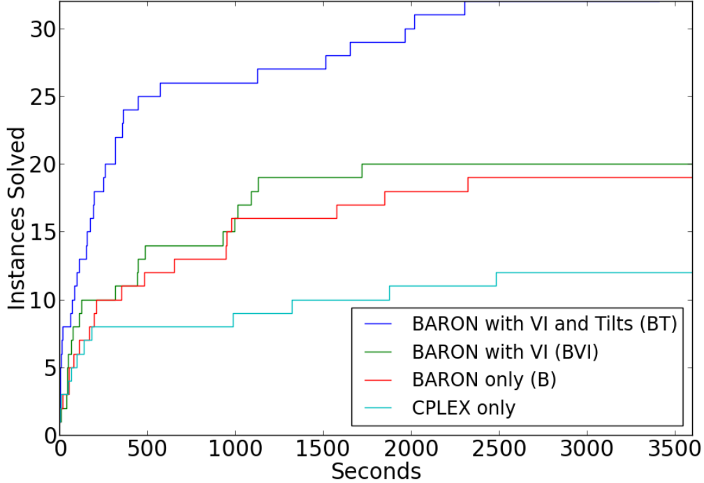
Figure 2: Cumulative distribution plots of solution times for the transportation problem. The plots from top to bottom correspond to the order of the labels in the legend.
