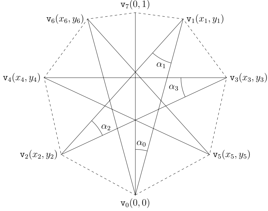
Figure 5: Definition of variables \alpha_0, \alpha_1, \dots, \alpha_{\frac{n}{2}-1} : Case of n = 8 vertices
