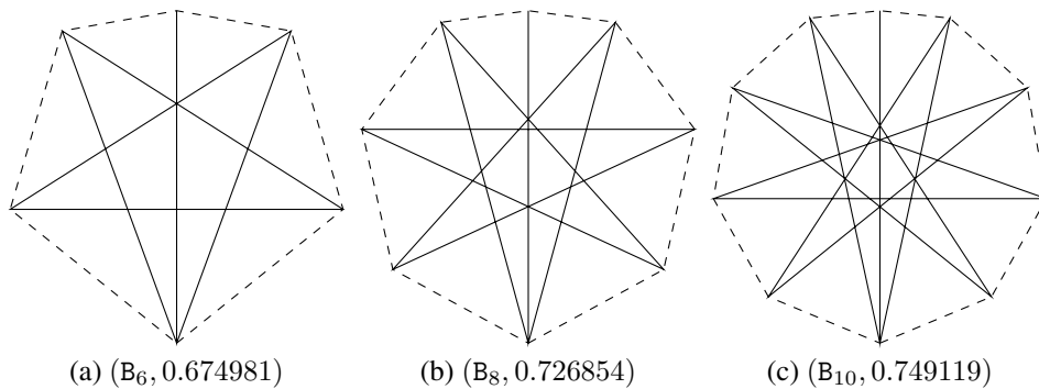
Figure 6: Polygons (B_n, A(B_n)) defined in Theorem 1
