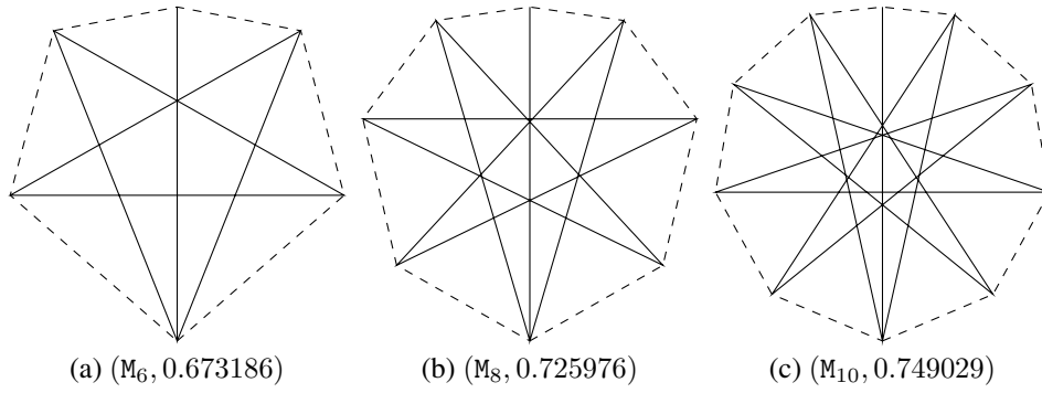
Figure 4: Mossinghoff polygons (M_n, A(M_n))
